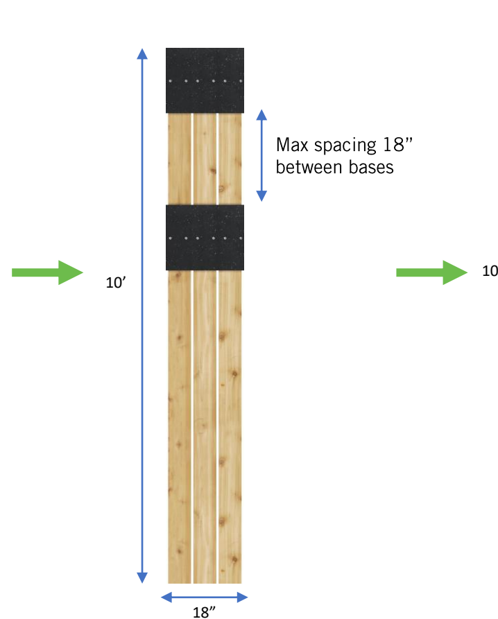
Fig 2. Space the bases max 18" apart.
