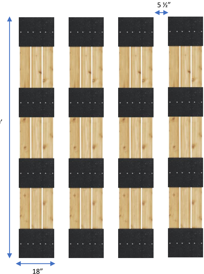
Fig 3. Build four identical panels.
