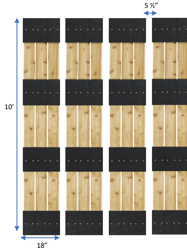
Fig 4. Arrange the panels 5 ½" apart.
